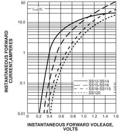
Fig. 2 TYPICAL INSTANTANEOUS FORWARD
