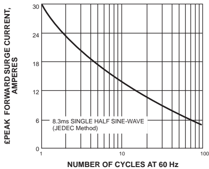
Fig. 5- MAXIMUM NON - REPETITIVE SURGE CURRENT
