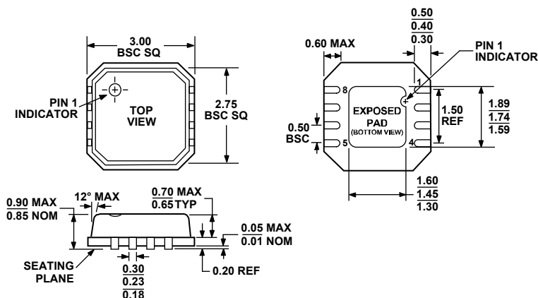
Figure 53. 8-Lead Lead Frame Chip Scale Package [LFCS_VD] 3 mm x 3 mm Body, Very Thin, Dual Lead (CP-8-2)
