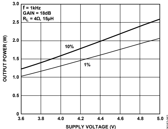
Figure 24. Maximum Output Power vs. Supply Voltage, R_L = 4 \Omega , A_V = 18 \text{ dB}
