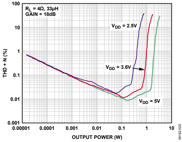
Figure 3. THD + N vs. Output Power into 4 Ω, A_V = 18\text{ dB}
