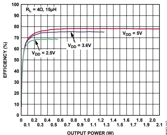
Figure 25. Efficiency vs. Output Power into 4 \Omega
