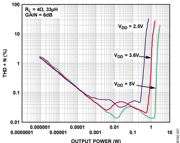
Figure 5. THD + N vs. Output Power into 4 Ω, A_V = 6\text{ dB}
