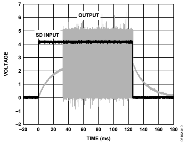
Figure 36. Turn-Off Response
