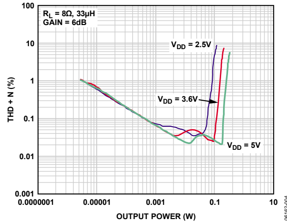
Figure 6. THD + N vs. Output Power into 8 Ω, A_V = 6\text{ dB}
