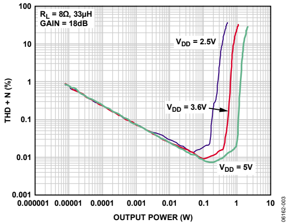
Figure 4. THD + N vs. Output Power into 8 Ω, A_V = 18\text{ dB}
