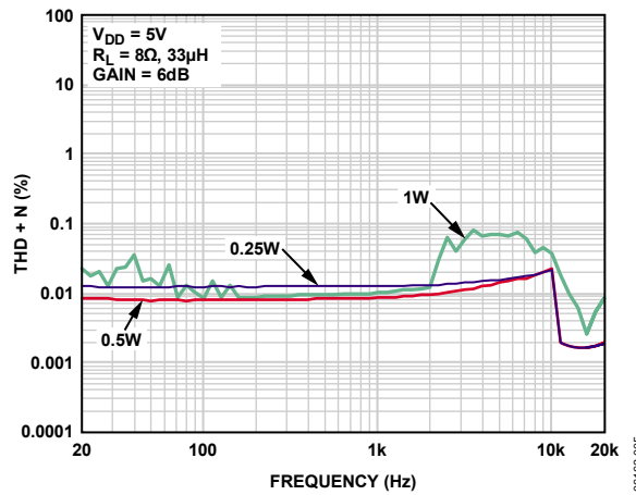
Figure 7. THD + N vs. Frequency, V_{DD} = 5\text{ V} , R_L = 8\Omega , A_V = 6\text{ dB}
