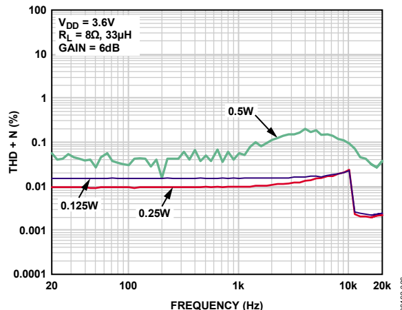
Figure 8. THD + N vs. Frequency, V_{DD} = 3.6\text{ V} , R_L = 8\Omega , A_V = 6\text{ dB}
