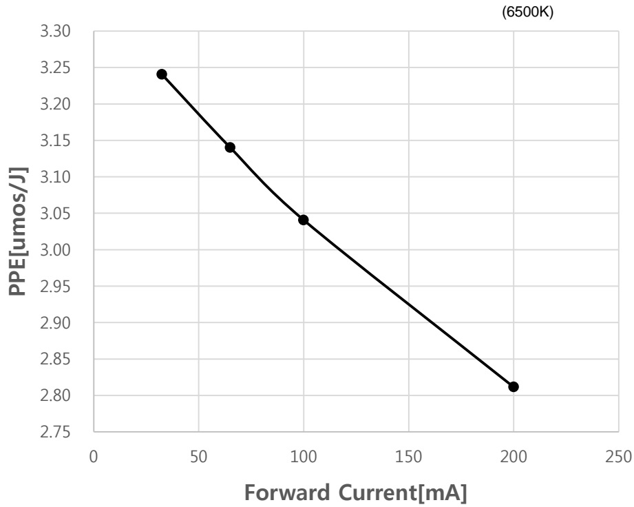
Fig 11. Forward Current vs. Photosynthetic Photon Energy , T_j = 25^\circ\text{C}
