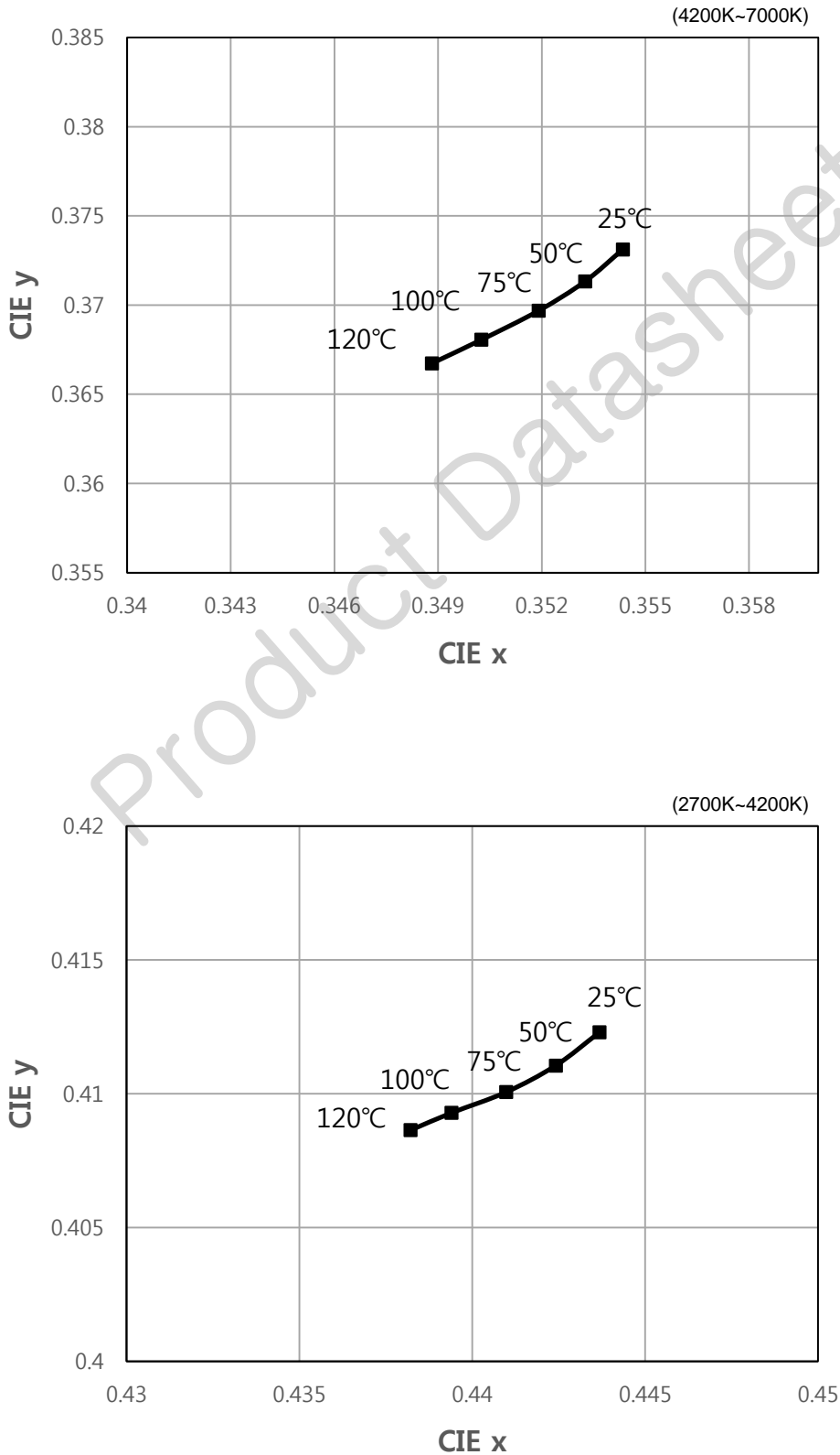
Fig 8. Chromaticity Coordinate vs. Junction Temperature, I_F=65mA
