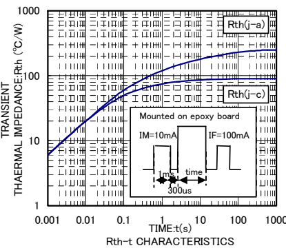
R_{\theta-t} CHARACTERISTICS
