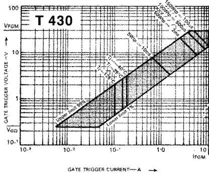
GATE CHARACTERISTICS
