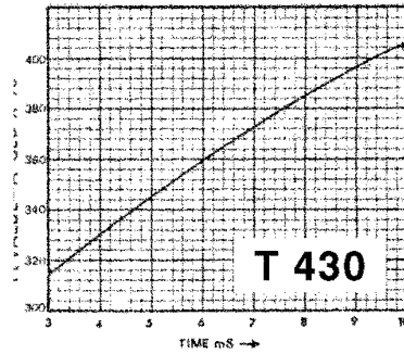
I 2 t VERSUS TIME AT 125°C
