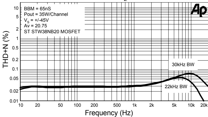
THD+N versus Frequency versus Bandwidth, R_L = 8\Omega
