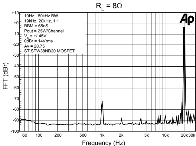
Intermodulation Performance R_L = 8\Omega
