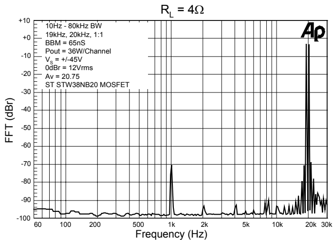
Intermodulation Performance R_L = 4\Omega
