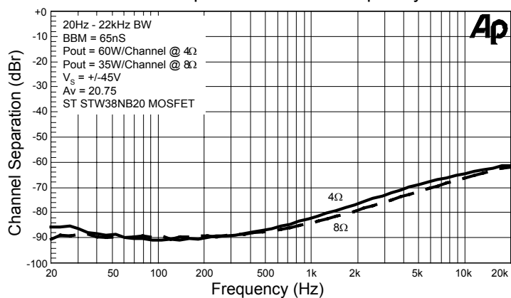
Channel Separation versus Frequency
