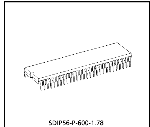
SDIP56-P-600-1.78 Weight : 5.55g (Typ.)
