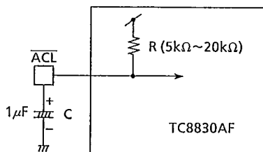
Fig.5.30 Power on reset circuit
