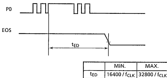
Fig.5.11 EOS delay time at manual control
