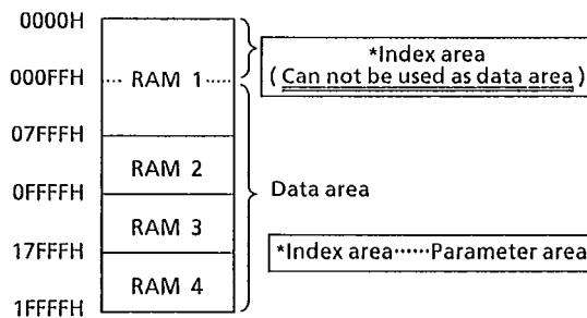
Fig.5.14 Memory map ( In case of 256K SRAM )
