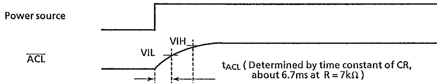
Fig. 5.31 \overline{ACL} input at power on reset
