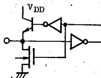
A. Bipolar Transistor LED Driver Built-in I/O.
