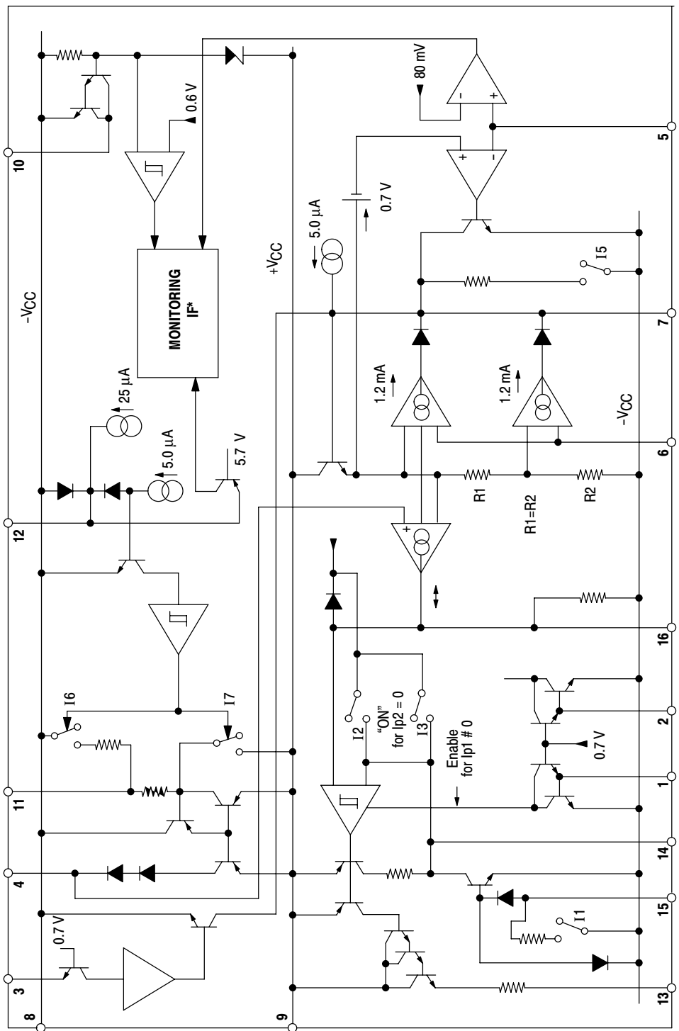
Figure 8. Simplified Schematic
