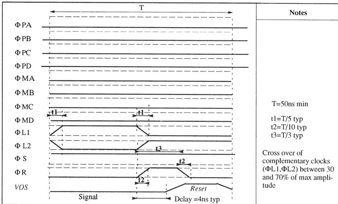
Figure 11. Horizontal Pixel Summation on ΦS Gate (Two Adjacent Pixel Summation)
