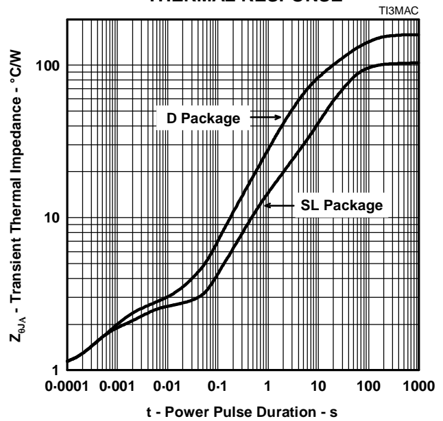
t - Power Pulse Duration - s Figure 12.
