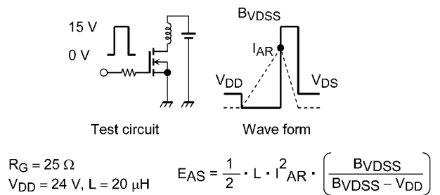
Fig. 8.16 Test Circuit/Waveform
