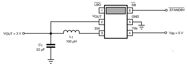
FIGURE 7: CONVERTER WITH STANDBY
