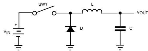
FIGURE 1: SIMPLE "BUCK" CONVERTER
