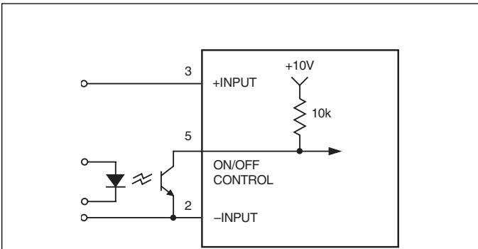
Figure 6. Driving the On/Off Control Pin
