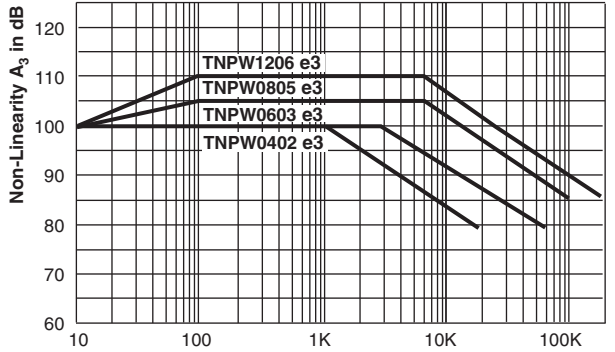
Non-Linearity
