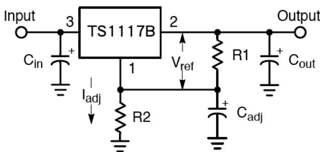
Adjustable Output Voltage Version
