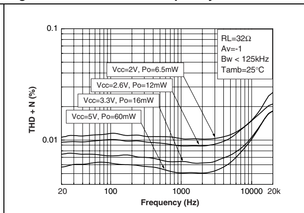
Figure 54. THD + N vs. frequency
