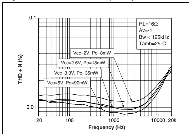
Figure 53. THD + N vs. frequency
