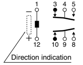
Schematic (Bottom view) Single side stable 1 coil latching
