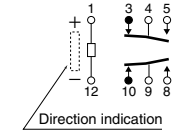
Schematic (Bottom view) Single side stable 1 coil latching
