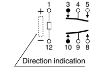
Schematic (Bottom view) Single side stable 1 coil latching
