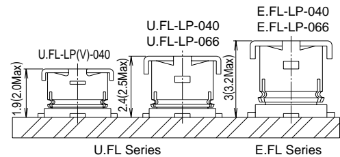
Mated Height Comparison (With Hirose Product)
