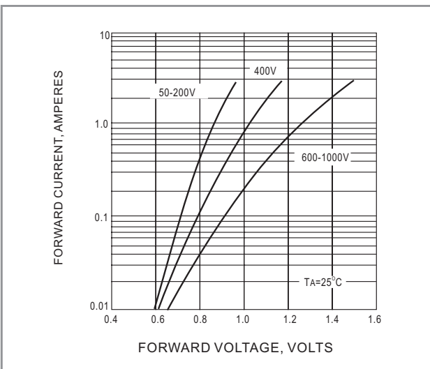
Fig.3 FORWARD CHARACTERISTICS
