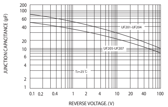
FIG.6-TYPICAL JUNCTION CAPACITANCE
