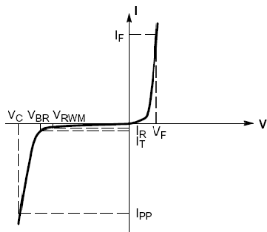
Uni-Directional TVS
