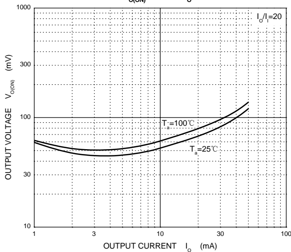
V_{0(ON)} — I_o
