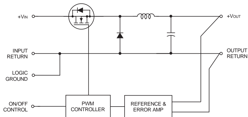
Figure 1. Simplified Schematic
