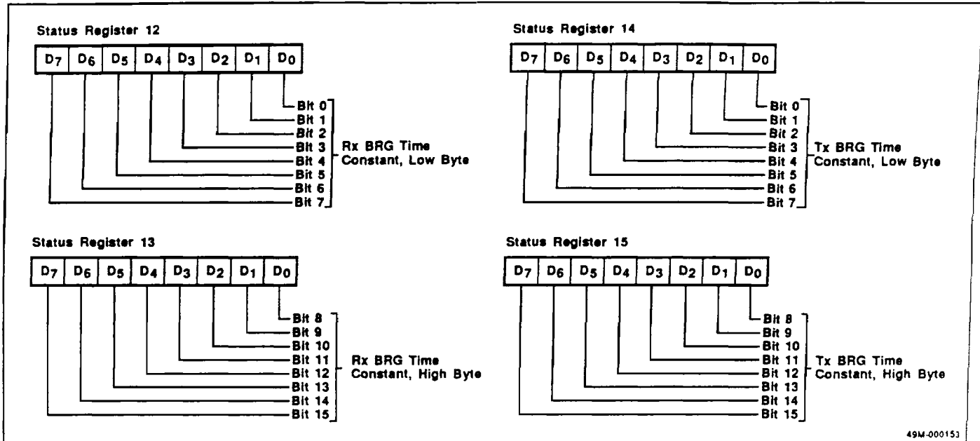
Figure 5. Status Register Bit Functions (cont)
