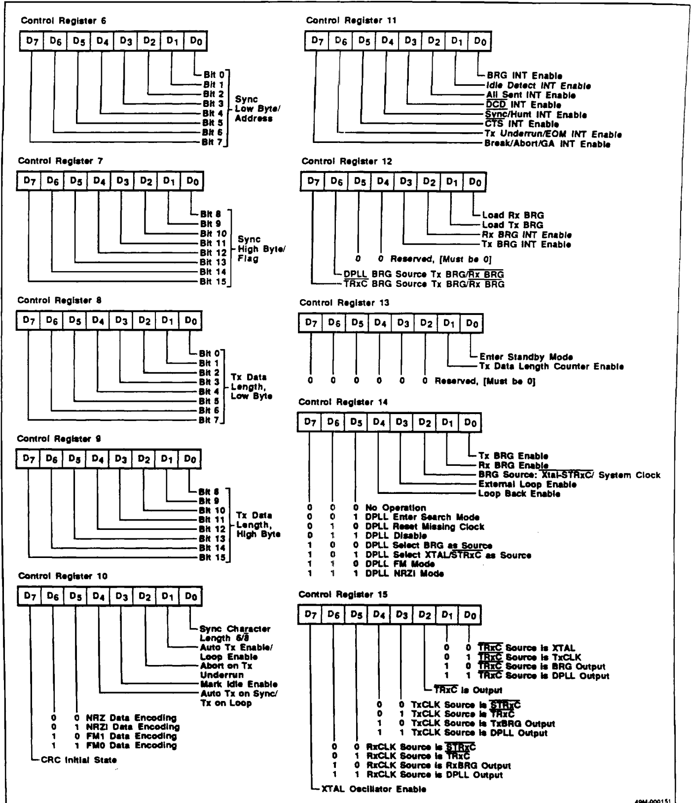
Figure 4. Control Register Bit Functions (cont)
