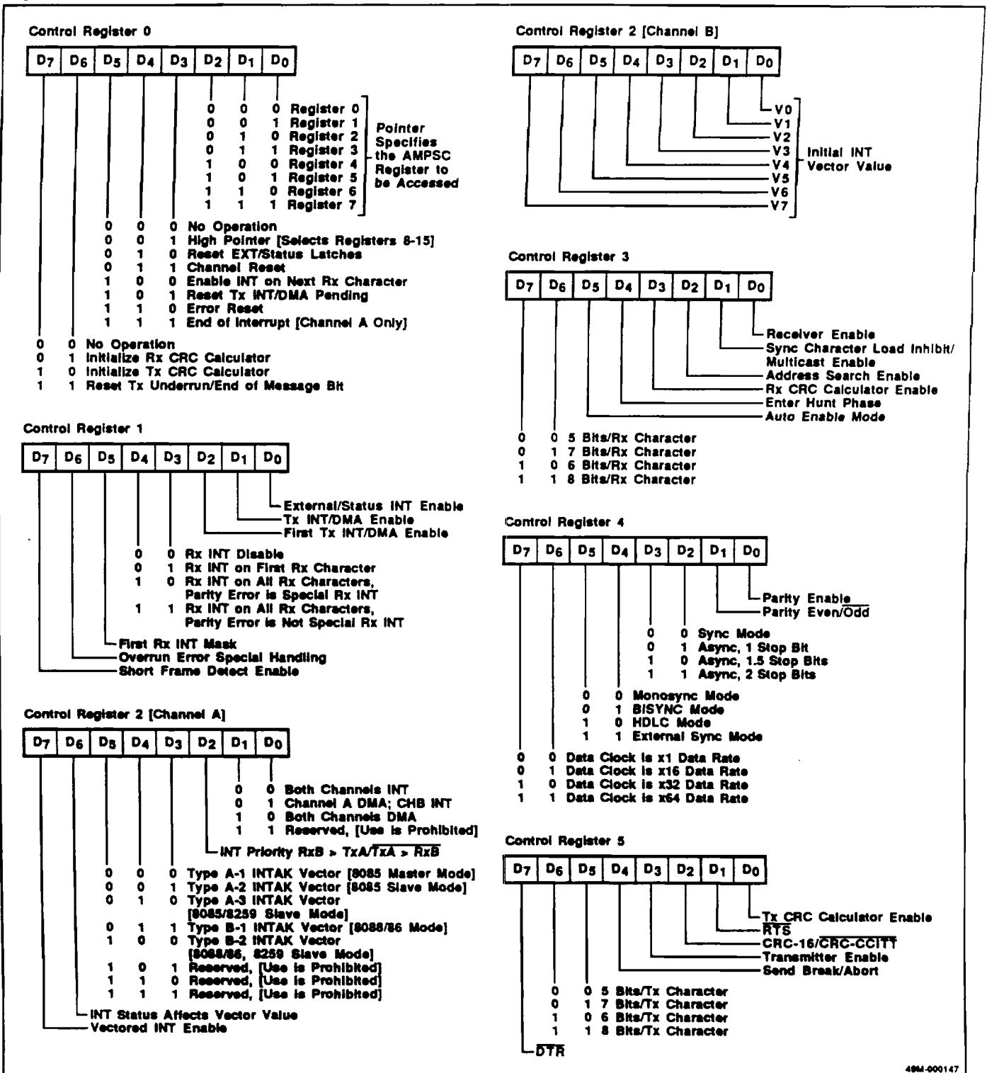
Figure 4. Control Register Bit Functions
