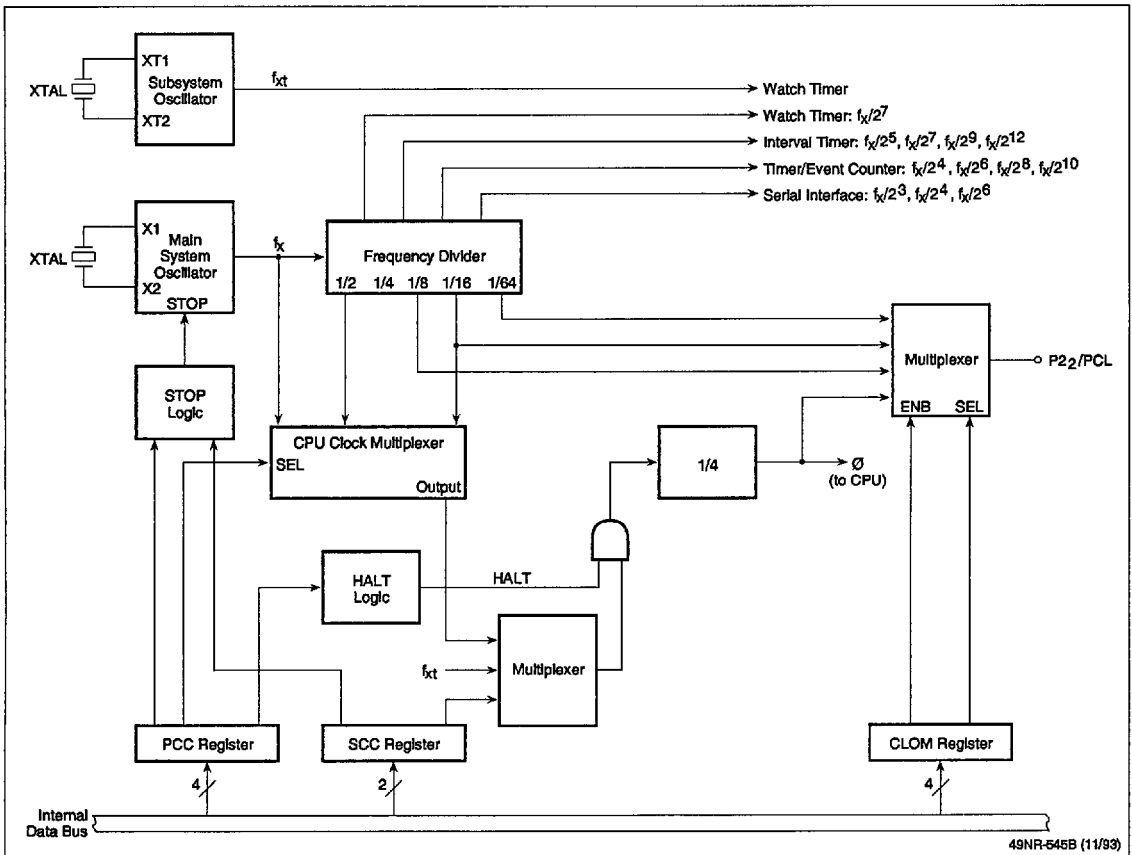
Figure 7. Clock Generator
