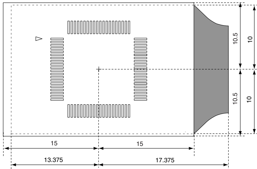
Figure B-12. For 80-Pin GK Package
