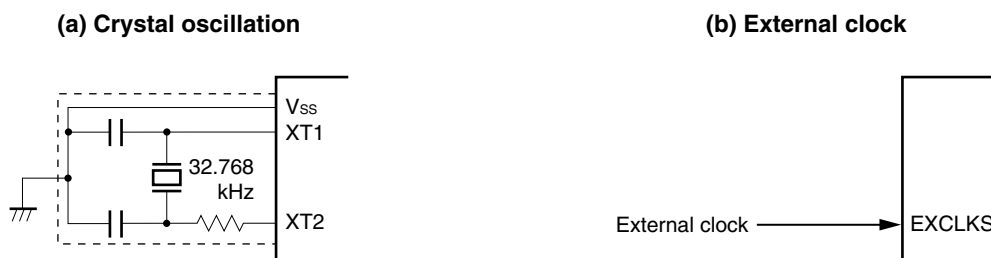
Figure 6-13. Example of External Circuit of XT1 Oscillator
