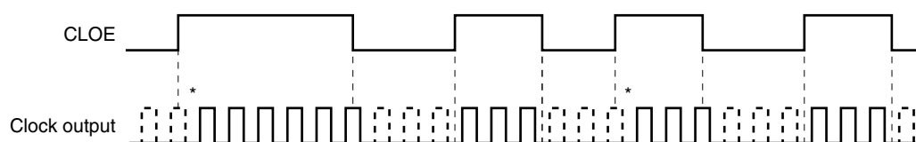
Figure 12-6. Remote Control Output Application Example
