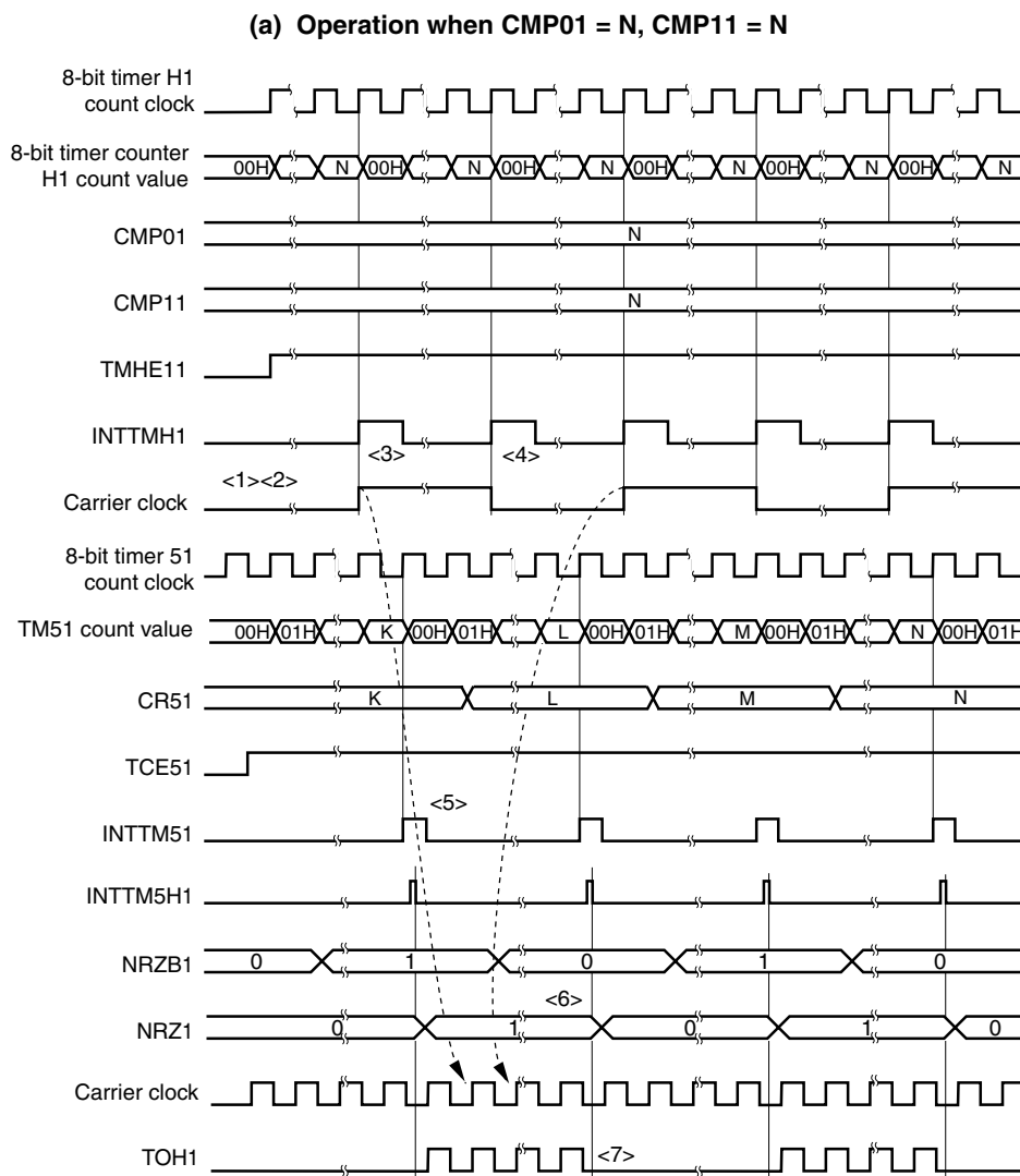
Figure 9-15. Carrier Generator Mode Operation Timing (1/3)
