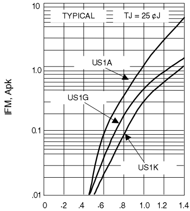
Fig. 2-FORWARD CHARACTERISTICS
