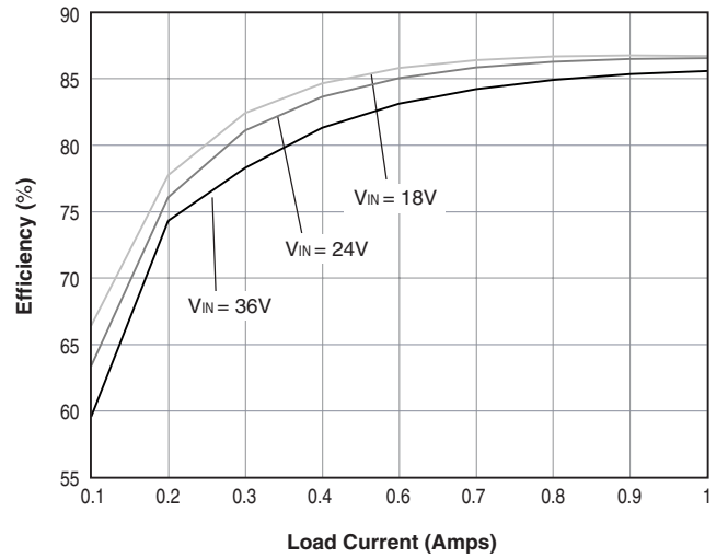
UWR-15/1000-D24A Efficiency vs. Line and Load
