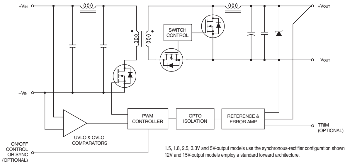
Figure 1. Simplified Schematic
