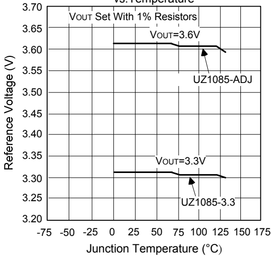
Figure 5. Output Voltage vs. Temperature
