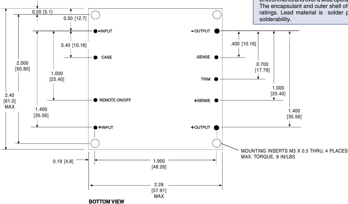
BOTTOM VIEW
