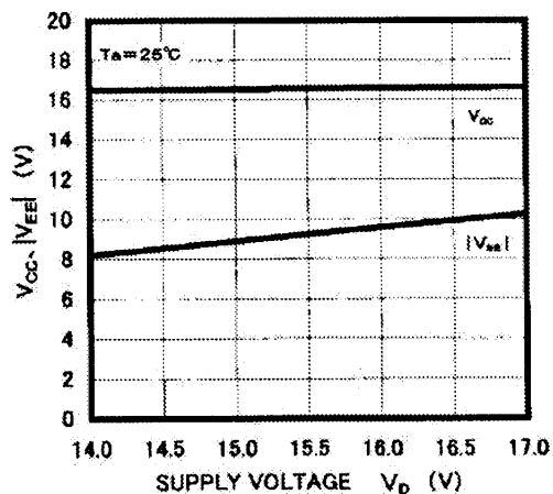
V CC , |V EE | - V D CHARACTERISTICS (TYPICAL)
