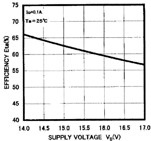
η drive - V D CHARACTERISTICS (TYPICAL)
