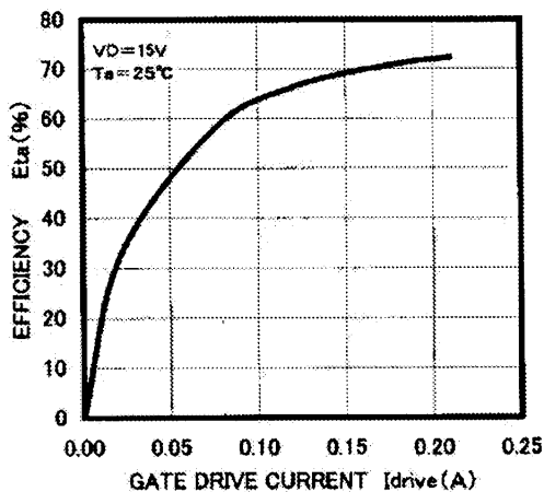
η drive - I drive CHARACTERISTICS (TYPICAL)
