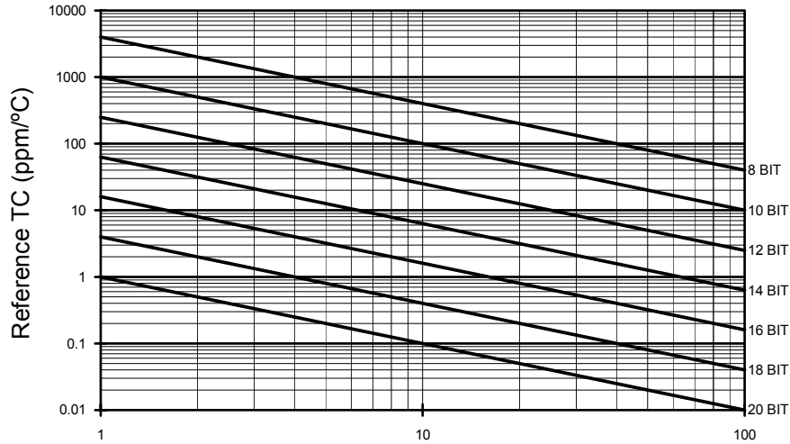
Reference TC vs. ΔT change from 25°C for 1 LSB change
