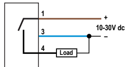
3-Pin PNP Models
