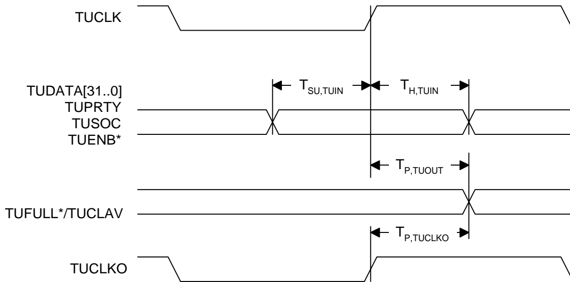
Figure 4: Tx UTOPIA Interface Timing Dependencies
