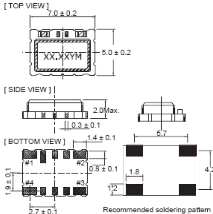
Figure 3, Package drawing
