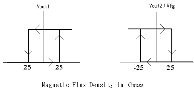
WSH41FC Complementary Output1 vs.Output2/Vfg
