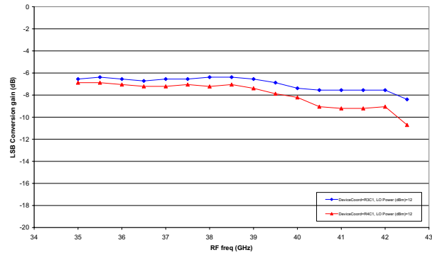
3_0058: LSB Conversion gain (dB) vs. RF freq (GHz) Vg = -1.1V, LO = 12dBm, IF = 3GHz
