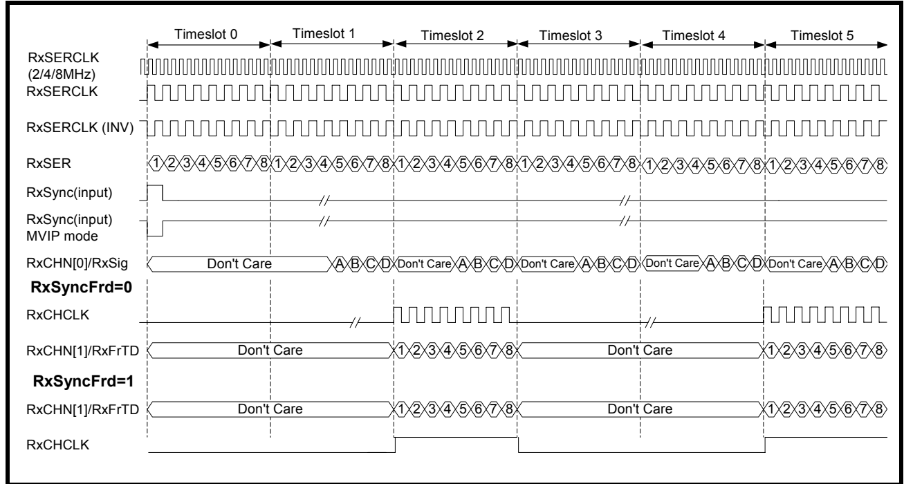
FIGURE 71. WAVEFORMS FOR CONNECTING THE RECEIVE NON-MULTIPLIED HIGH-SPEED INPUT INTERFACE AT MVIP 2.048MBIT/S, 4.096MBIT/S, AND 8.192MBIT/S
