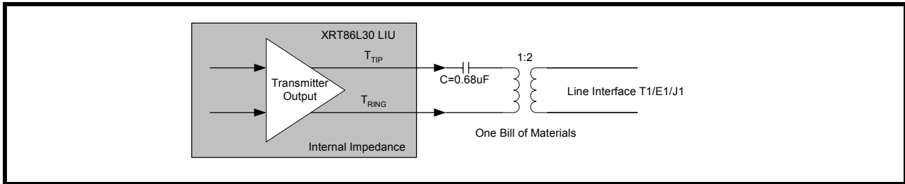
FIGURE 56. TYPICAL CONNECTION DIAGRAM USING INTERNAL TERMININATION
