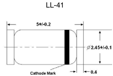
Glass case MELF Dimensions in mm
