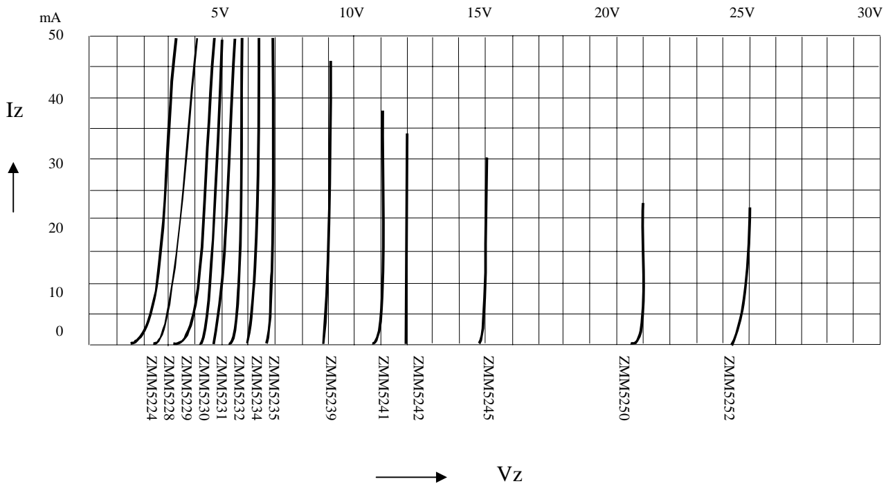
FIG.1- BREAKDOWN CHARACTERISTICS
