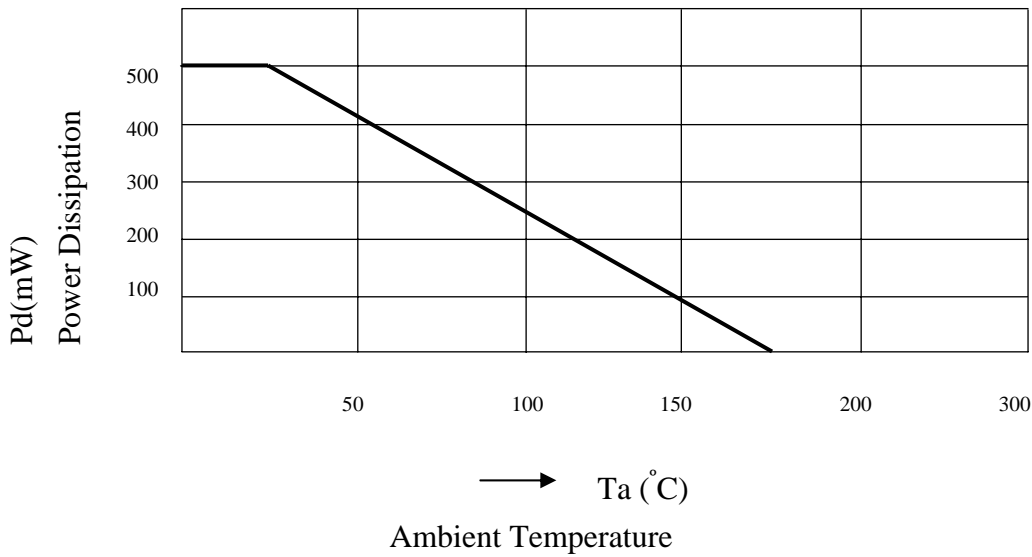
FIG.2- POWER, TEMPERATURE DERATING CURVE
