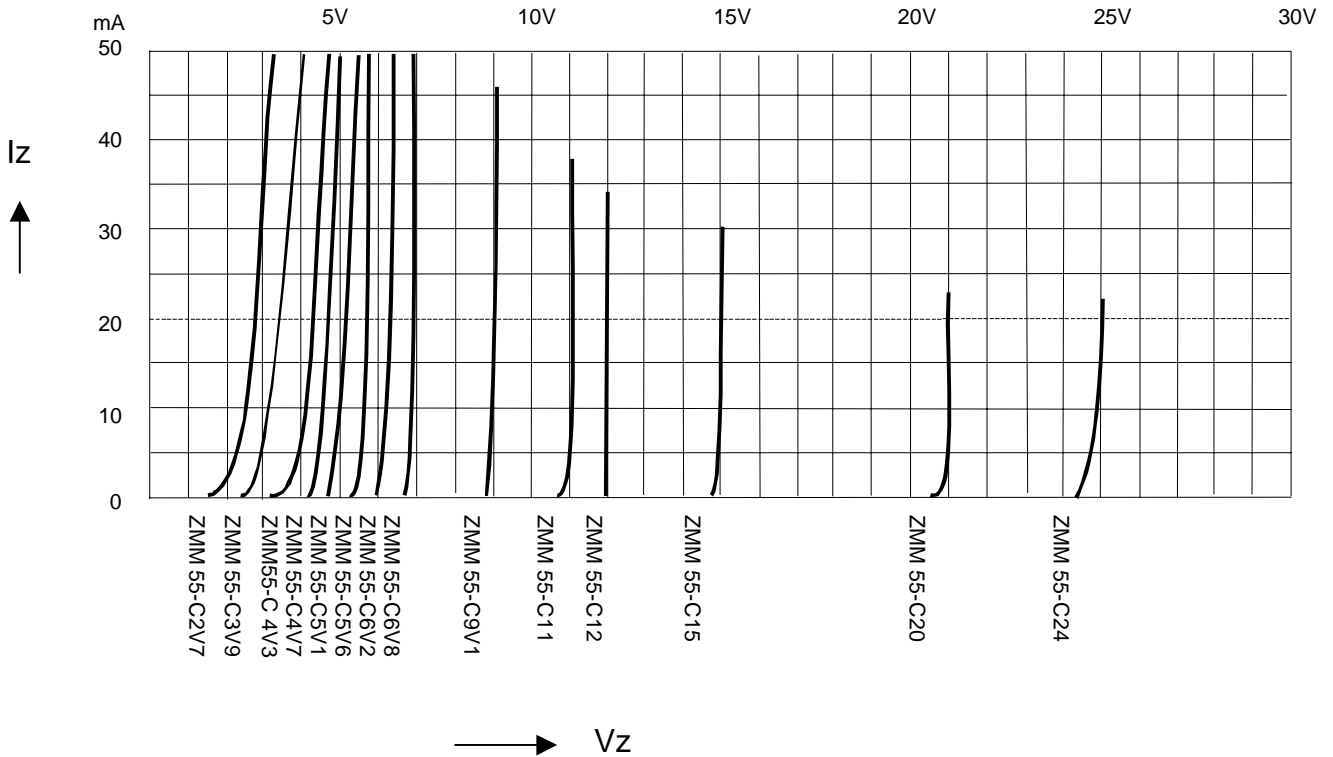
FIG.1- BREAKDOWN CHARACTERISTICS
