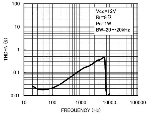
Fig. 2 THD+N - Frequency
