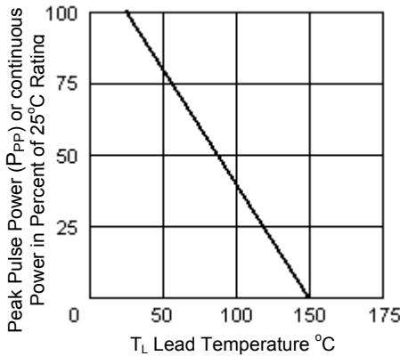
FIGURE 3 Derating Curve
